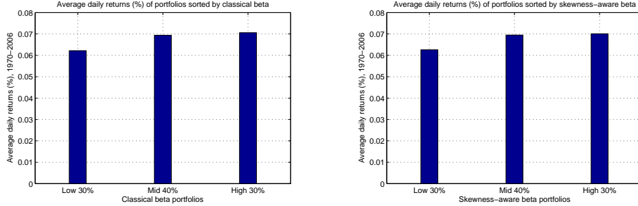
Figure 5: Bar charts of realized average returns for sorted portfolios according to classical beta and skewness-aware beta.
