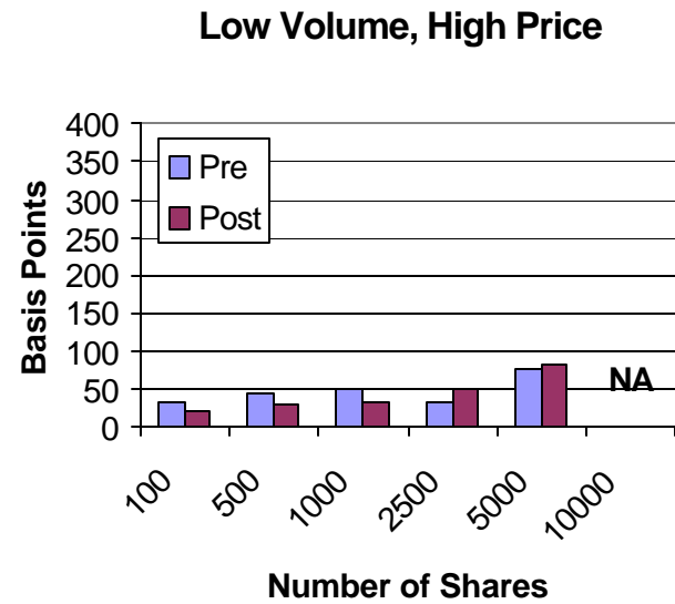
Fig. 3. The cost of demanding liquidity for orders with original order sizes of 100, 500, 1000, 2500, 5000, and 10,000 shares. The cost is measured as the cumulative percent mark-up of the average execution price(s) over the midpoint of the contemporaneous bid-ask quote at the time of submission.
