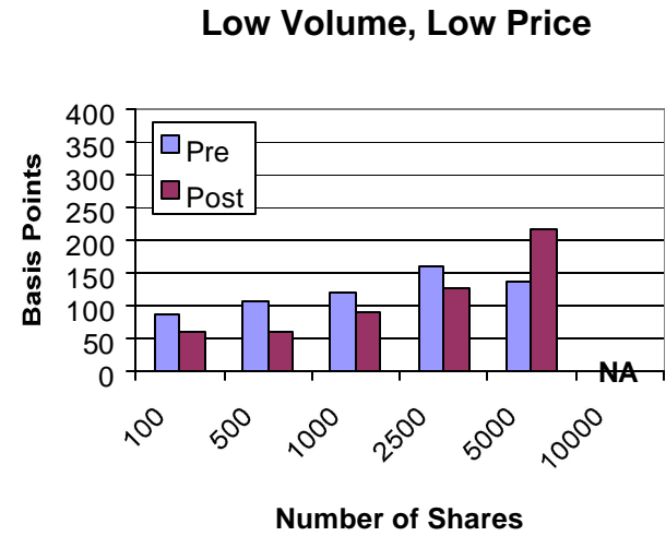
Fig. 3. The cost of demanding liquidity for orders with original order sizes of 100, 500, 1000, 2500, 5000, and 10,000 shares. The cost is measured as the cumulative percent mark-up of the average execution price(s) over the midpoint of the contemporaneous bid-ask quote at the time of submission.
